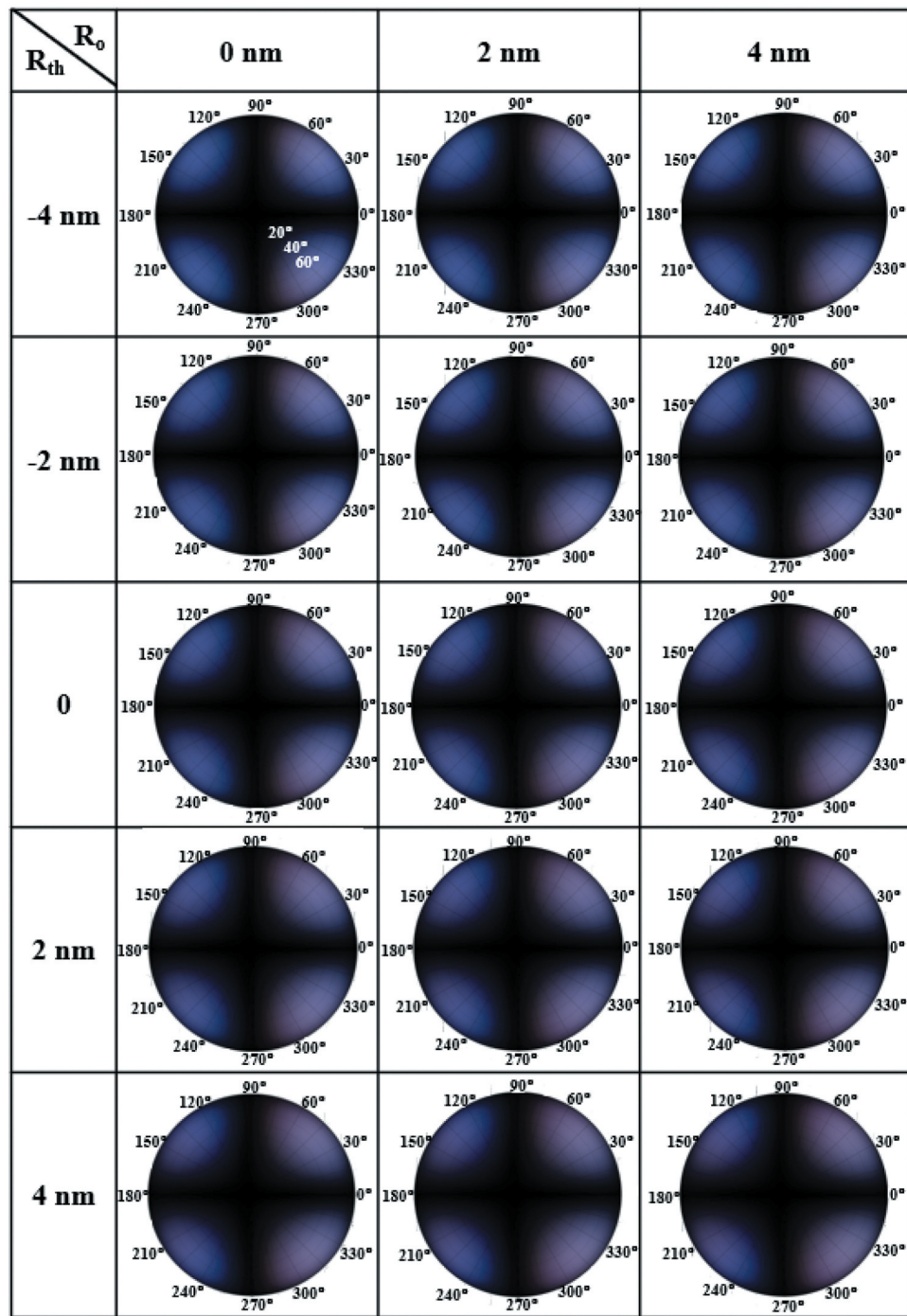
Figure 4. (Colour online) Calculated colour contour with brightness as a function of R_{th} and R_o of the front and rear TAC films in a dark state of the HA-LCD.
