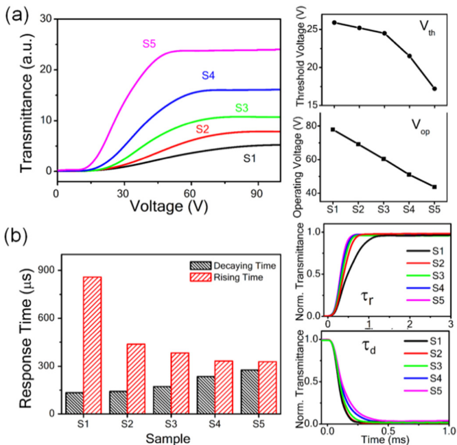
Fig. 4. (a) The voltage-dependent transmittance at 1 kHz square wave voltage. (b) The decaying and rising time of the prepared samples.
